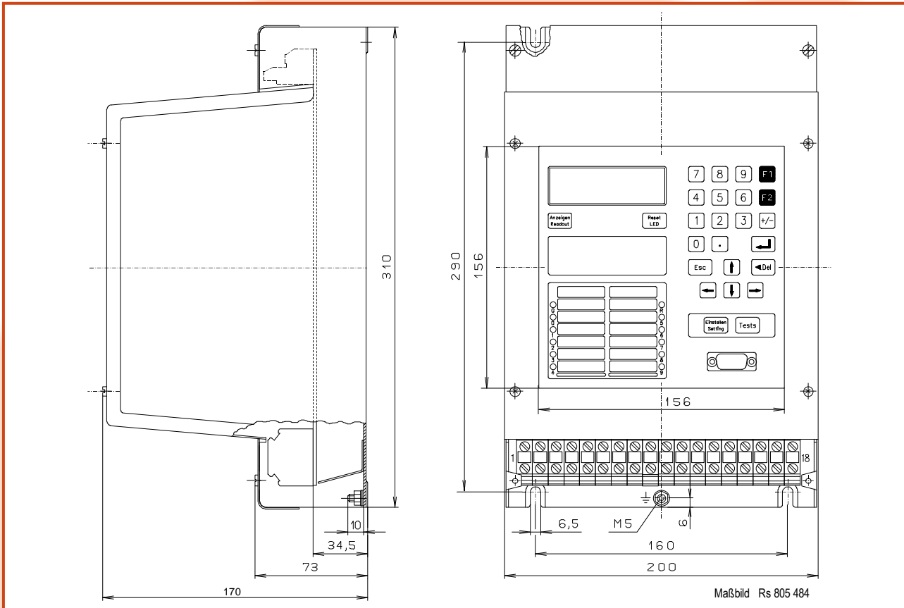
Fig. 9: DSRZW 2 housing for panel surface mounting, lower terminal cover not shown in top view. With the horizontal models the keypad is turned + or -90°.
