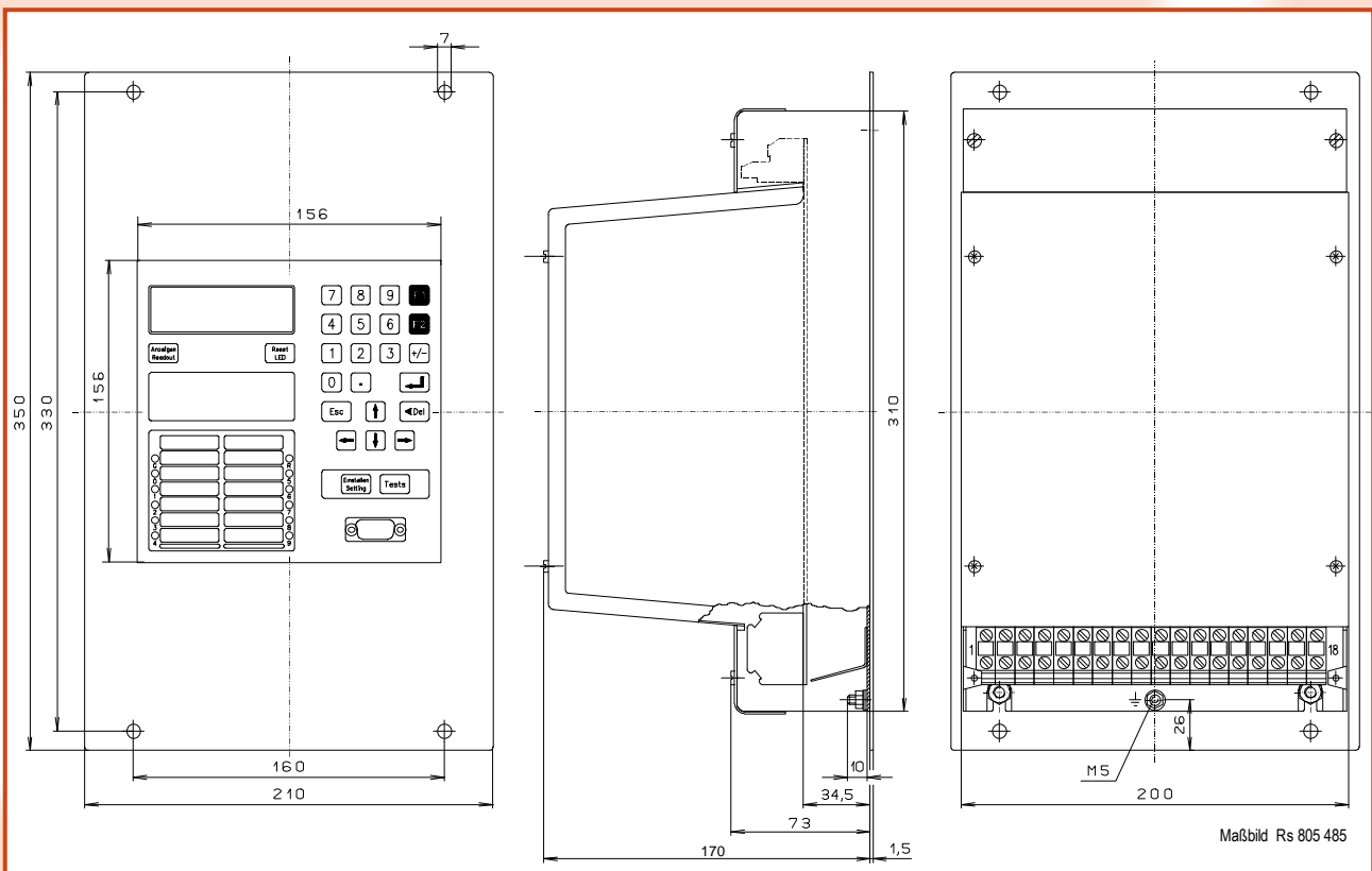
Fig. 10: DSRZW 2 housing for panel flush mounting, lower terminal cover not shown in rear view (right-hand side). The panel cut-out should be 202 mm * 312 mm when device will be put through from front side. With the horizontal models the keypad is turned + or -90°.
