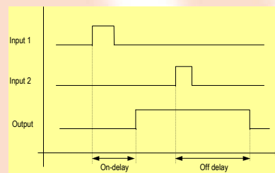
Fig. 8: Example for one effect of the pulse shaper stage
