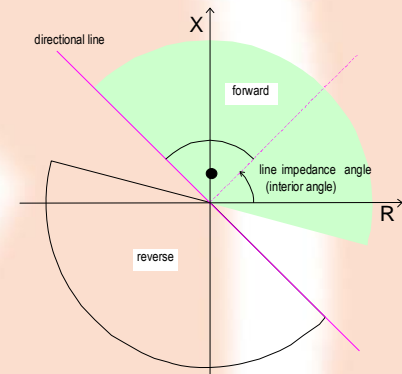
Fig. 6: Characteristic for determining the short-circuit directions
